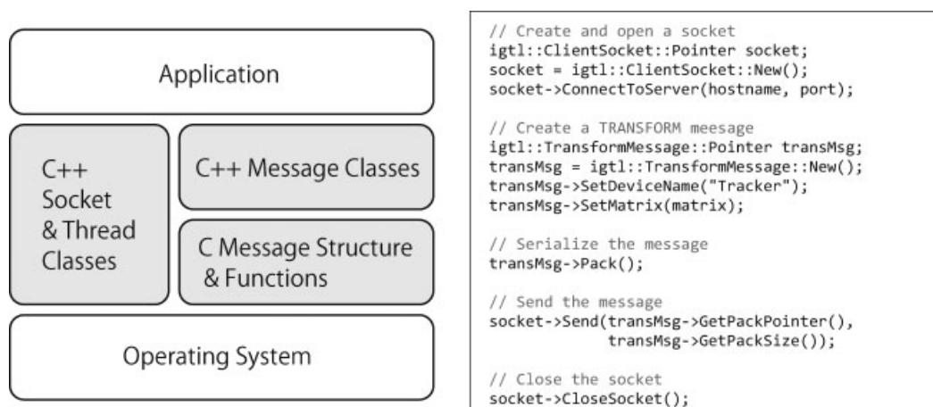
Figure 2. The structure of the OpenIGTLink Library (left) and an example code to send TRANSFORM data using the C++ message class and socket class (right). At the lowest level, the messages are defined as C structures with several supporting functions for message serialization. On top of the C structures and function, C++ message classes are built to provide an easier, safer and more extensible way to access to OpenIGTLink messages. As shown in the example code, the message classes have several access functions to set parameters for both message header and body, and a function to serialize the message and body. Besides message classes, multi-platform C++ socket and thread classes are provided to support writing platform-independent application codes
