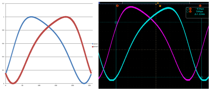
Fig. 3 Example waveforms for non-harmonic motors.
